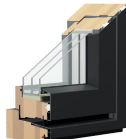
Figure 2: Top hung/ top swing/ side hung/ side swing window wooden with aluminium cladding
