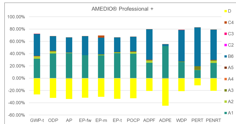
Figure 2 Percentage shares of the modules for selected environmental impact indicators over the life cycle
