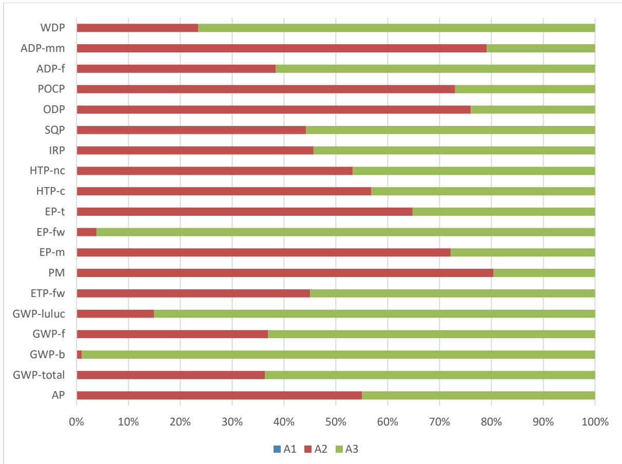
Figure 1 Shares of the product life phases in the environmental impacts for Crane® Spheres 10
